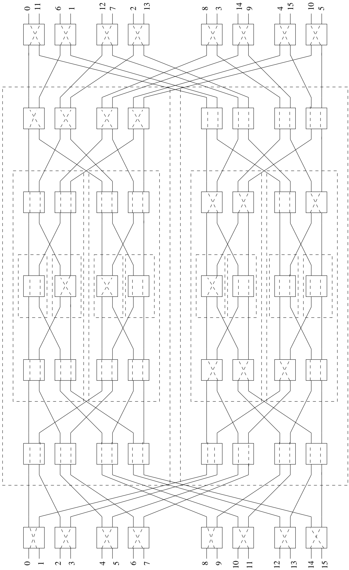
A 16x16 Benes Network (hw1_#1, one possible solution)
