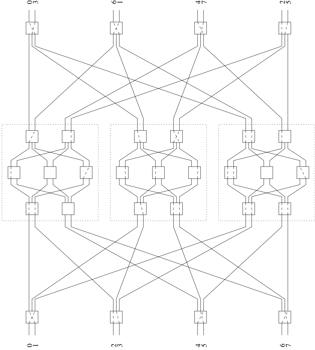
Non-rearrangeable non-blocking Clos network (hw1-#2, one possible solution)
