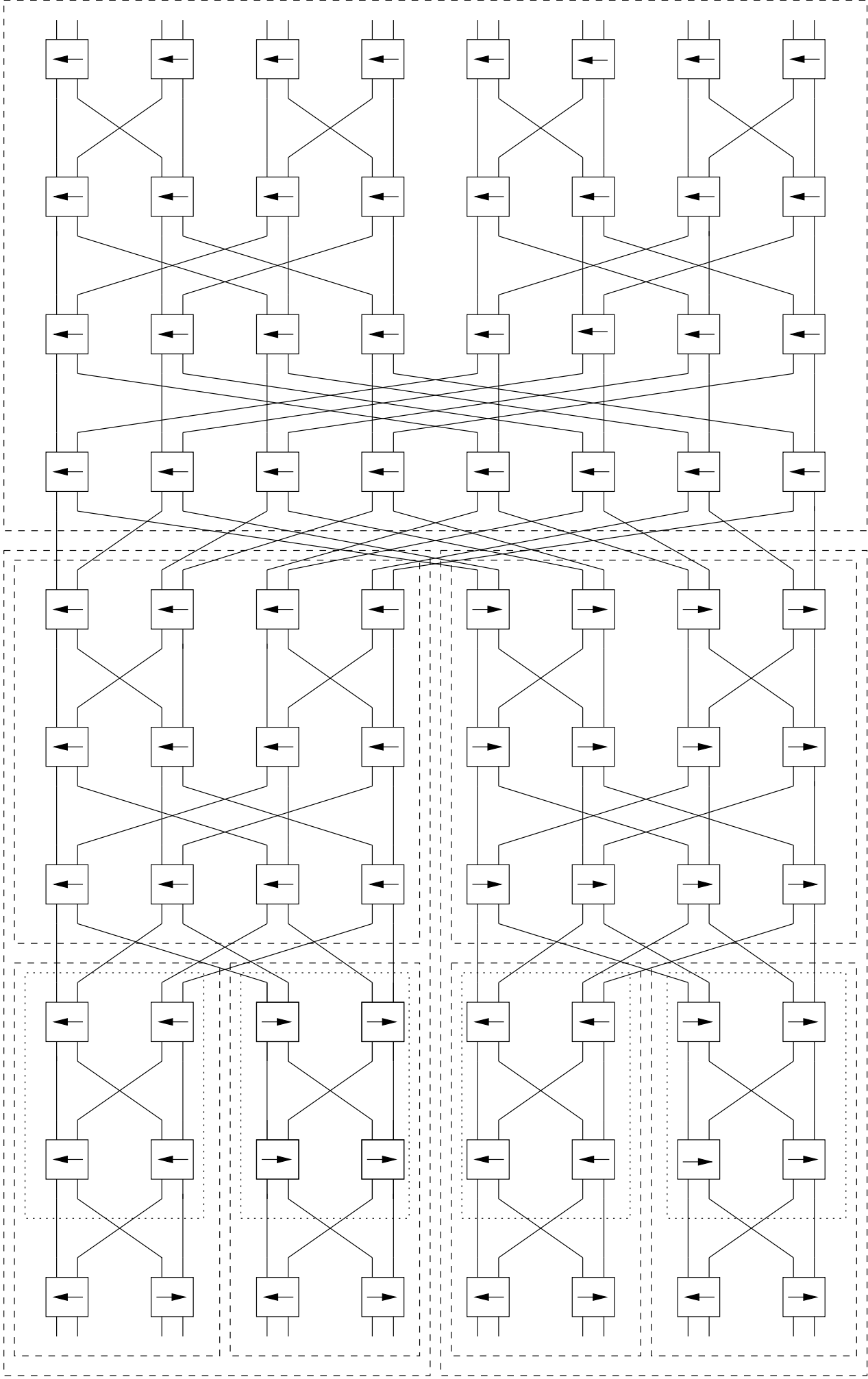
A 16-line Sorter Built Recursively Using Bitonic Sorters
